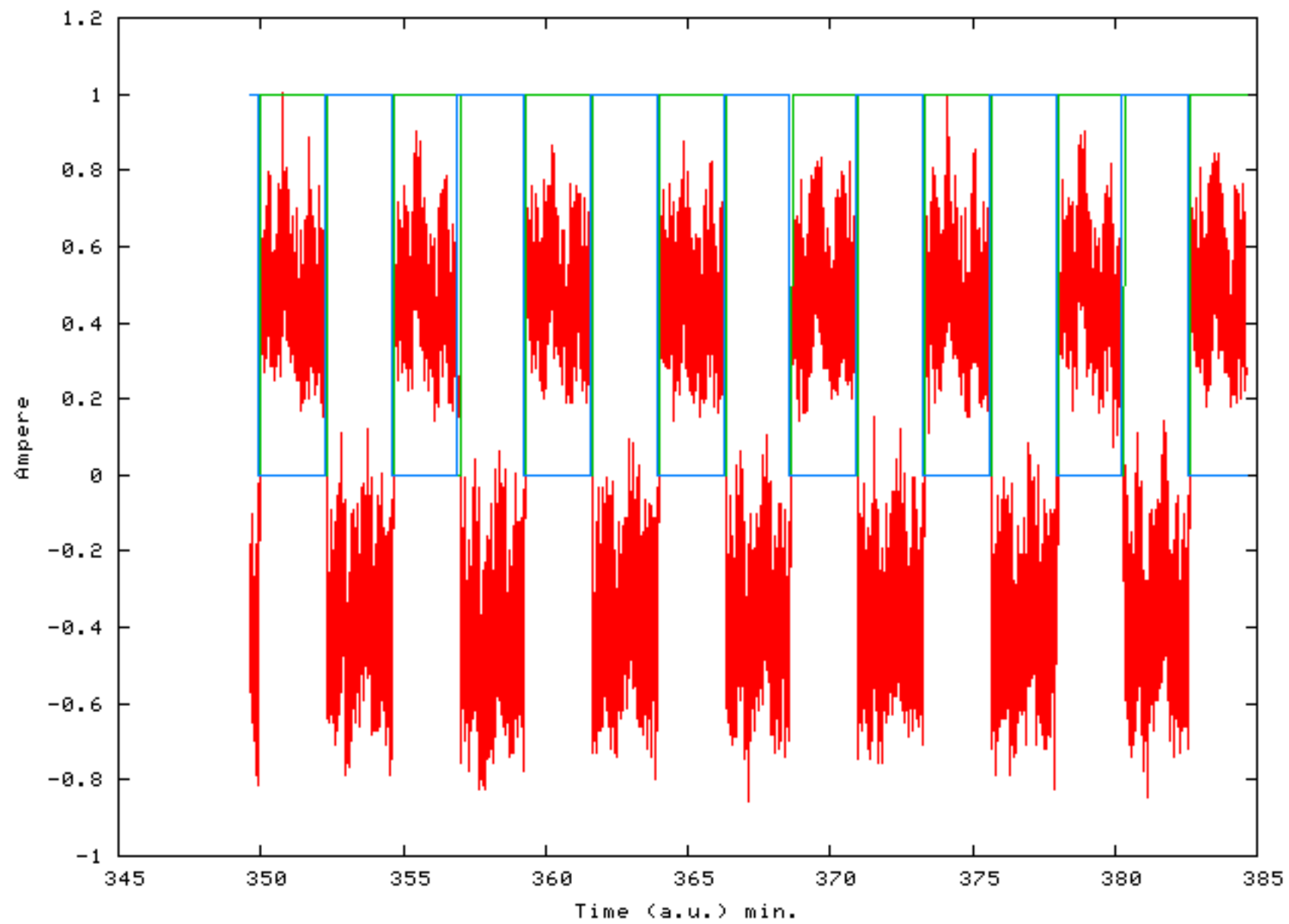
Current drawn by the motor shuttle (float)
